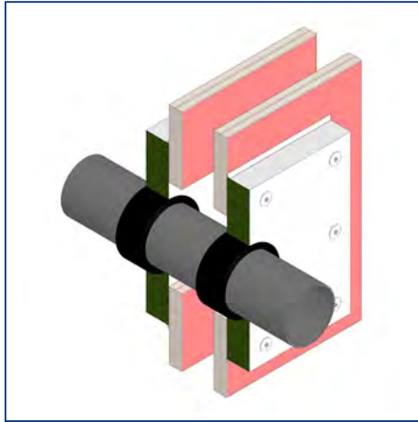
FB750 double batt pattern fit + FP302 Intustrap : up to EI120
